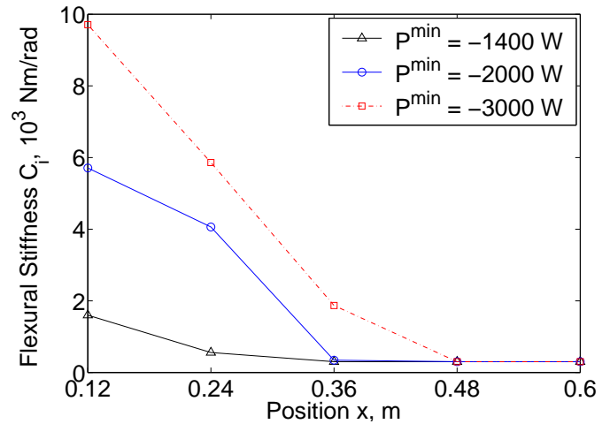
Fig. 4 Optimal stiffness distributions.
