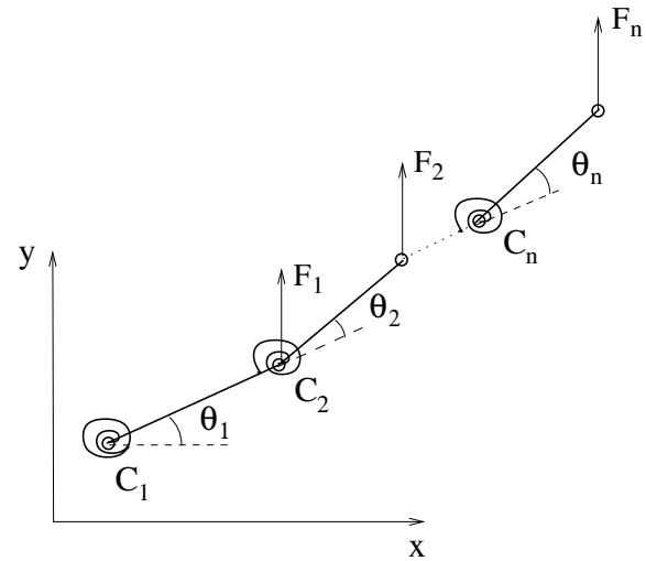
Fig. 15 2D bars system. All bars have length l , C_i is the stiffness of the i -th joint, the loads F_i are vertical.
