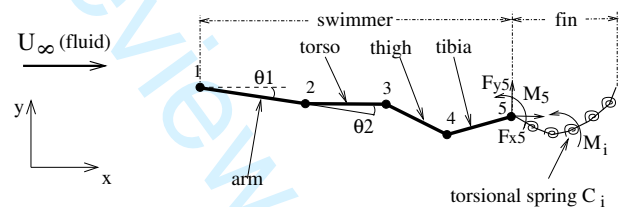
Fig. 2 Swimmer and monofin representation.
