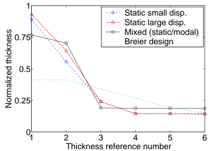
Fig. 13 Comparison among the three identification formulations and the Breier's monofin design.
