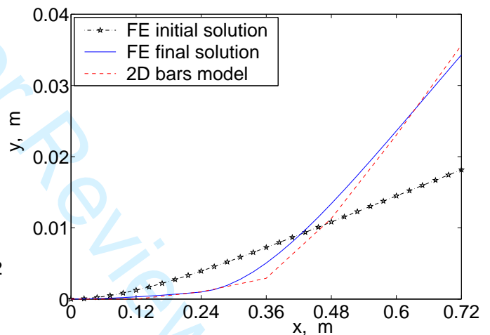
Fig. 14 Deformed shapes comparison for mixed formulation, load case 1.
