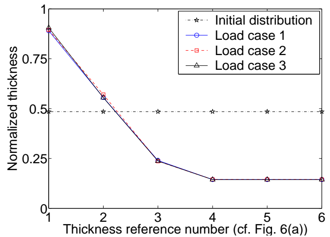
Fig. 8 Normalized identified thickness distributions for small displacements formulation.
