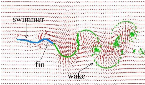
Fig. 3 Flow, swimmer and monofin visualization. Continuous trace, the obstacle; \times , the wake particles; \rightarrow , the relative velocity of the fluid.
