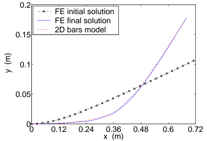
Fig. 11 Deformed shapes comparison for large displacements formulation, load case 1.
