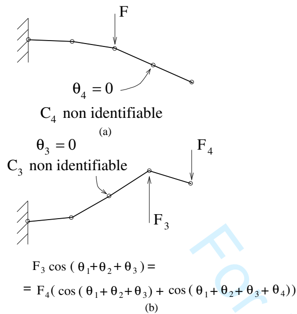
Fig. 16 Examples of loads such that the flexural stiffnesses are not identifiable, (a) the tip is not loaded, (b) moments cancel at joint 3.
