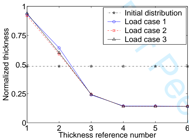
Fig. 10 Normalized identified thickness distributions for large displacements formulation.
