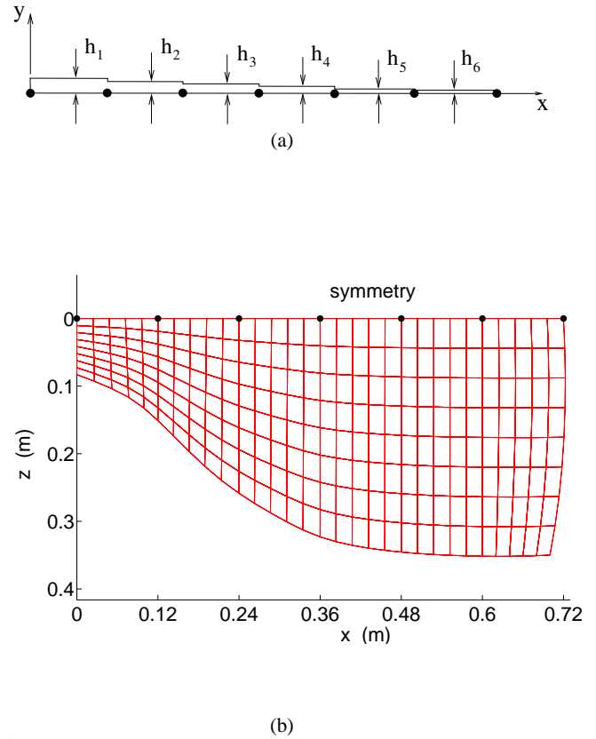
Fig. 6 Fin parameterization: thickness profile (a), half-planform shape and finite element mesh (b). The dots represent the NCP points where J_{static} is evaluated.
