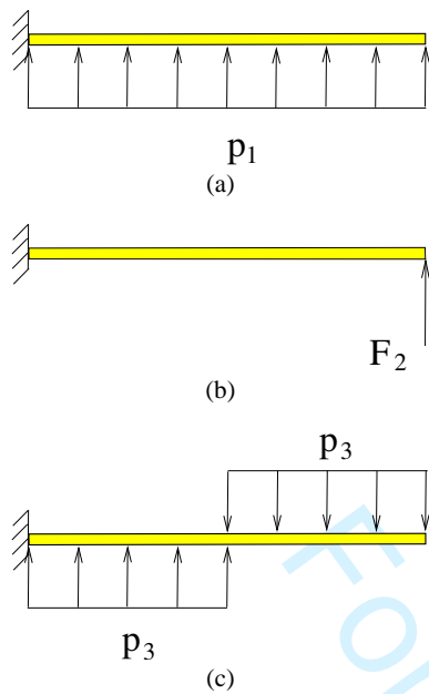
Fig. 7 The load cases considered for the thickness identification.
