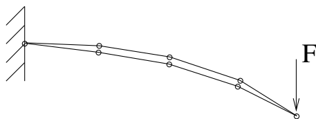
Fig. 17 Two deflected shapes that have the same displacements at the tip. This illustrates why C_i 's would not be identifiable if there was only a control point at the tip.
