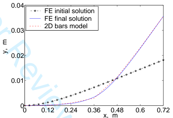
Fig. 9 Deformed shapes comparison for small displacements formulation, load case 1.
